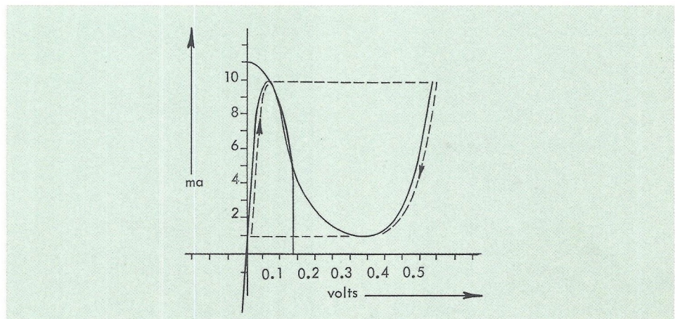
Figure 12 AC and DC load lines of tunnel diode in Figure 11 (B) superimposed on a 10-ma tunnel-diode curve.
