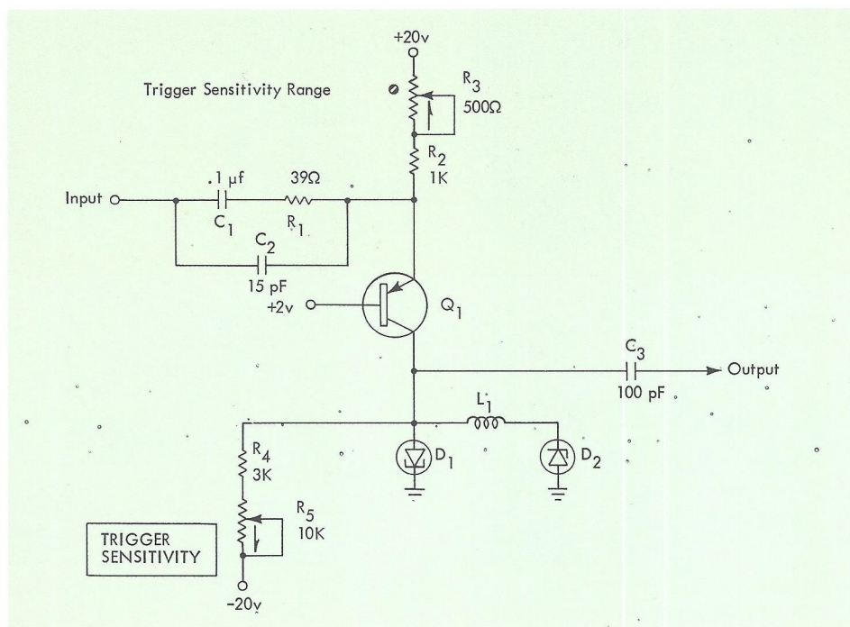
Figure 13 A few refinements to the circuit in Figure 11 (B) are included in the circuit shown here. See text for explanation.
