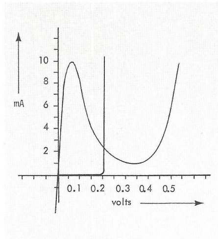
Figure 8 Curve of a hypothetical 200-mA zener diode superimposed on a 10-mA tunnel-diode curve.
