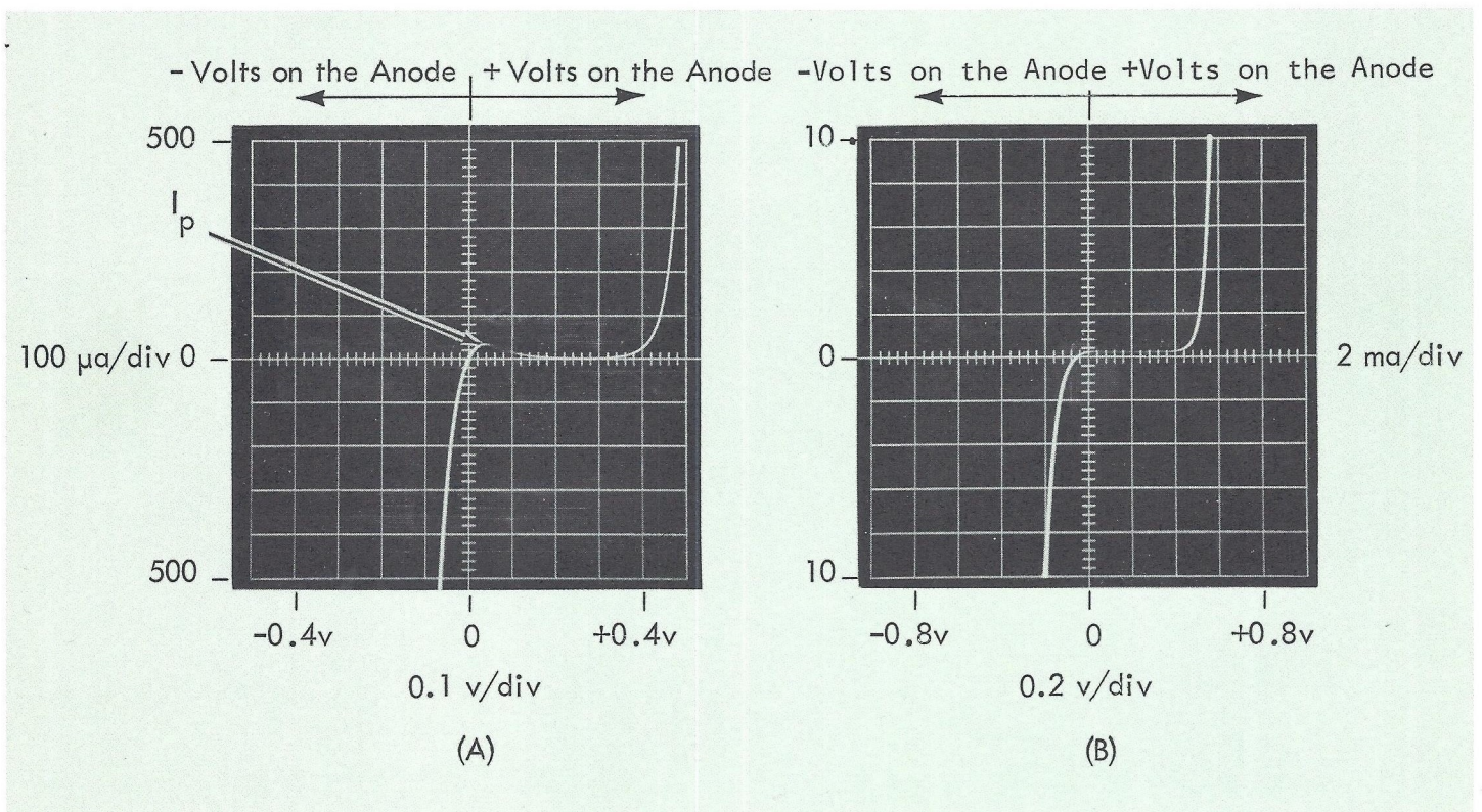
Figure 9 (A) Waveform photo showing peak current of a BD-4 back diode.
