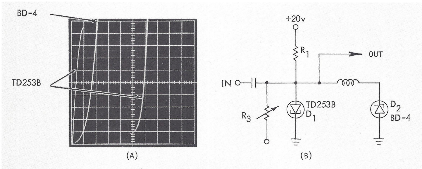
Figure 11 (A) Curves of a TD253B tunnel diode and a BD-4 back diode superimposed.
