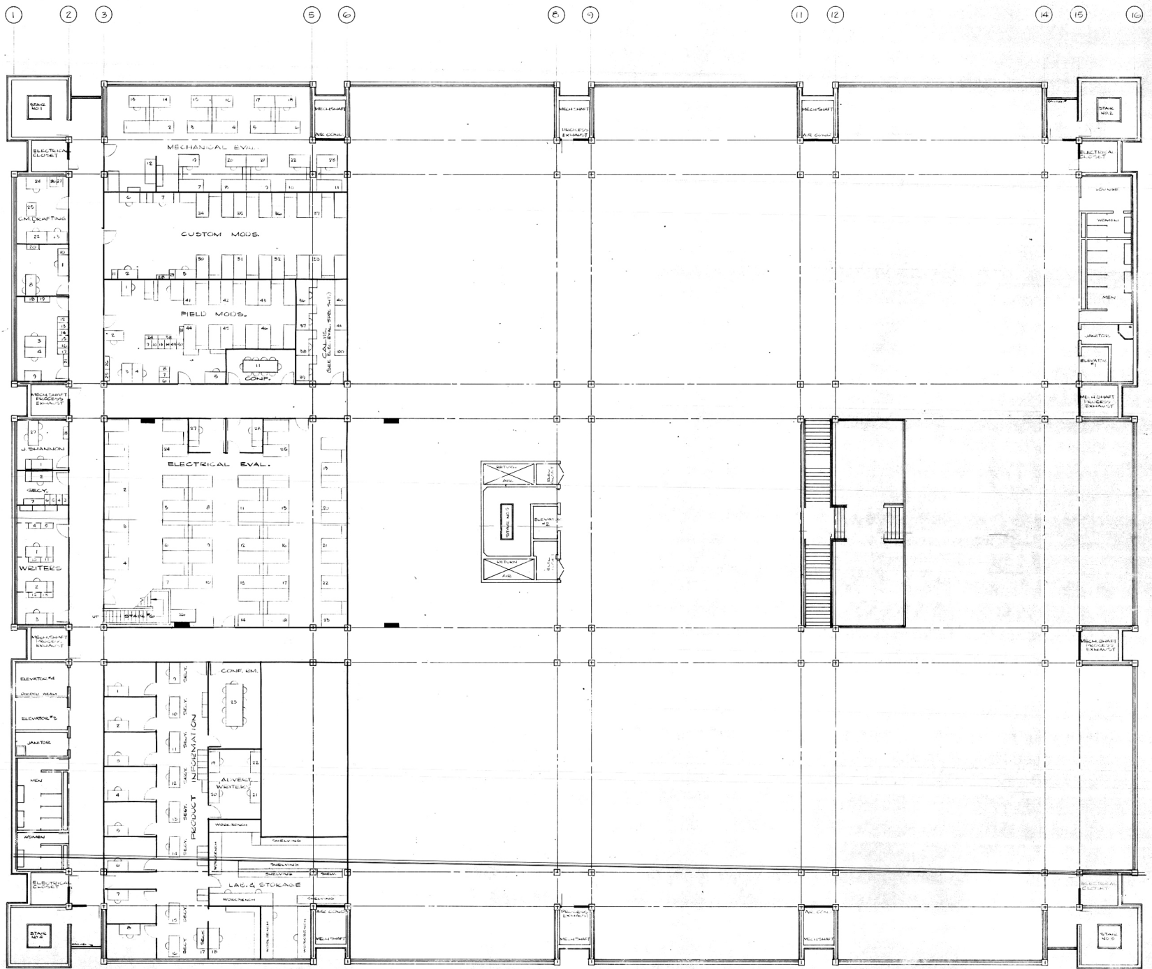
FOURTH LEVEL PLAN BUILDING NO. 50
